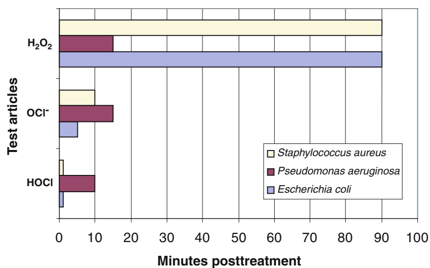
Figure 3. Comparative time kill studies of HOCl, NaOCl, and \text{H}_2\text{O}_2 against 3 test organisms— Escherichia coli 25922, Pseudomonas aeruginosa 27853, and Staphylococcus aureus 29213—at room temperature for total of 90 minutes.
